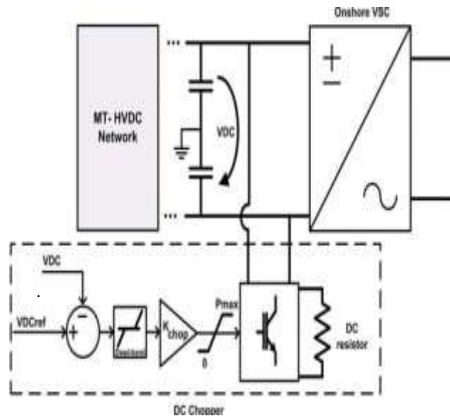
Figure 4. Control scheme of onshore dc chopper resistor
