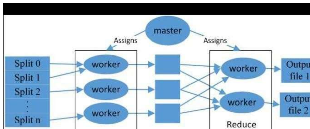
MapReduce flow
